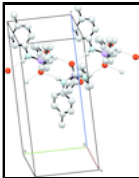
Fig. 2. Part of the crystal structure of the title compound with hydrogen bonding shown as dotted lines (the C—H hydrogen atoms are omitted for clarity).
