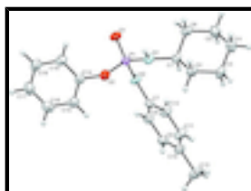
Fig. 1. The molecular structure of the title compound with ellipsoids shown at the 50% probability level. The disorder is not shown.
